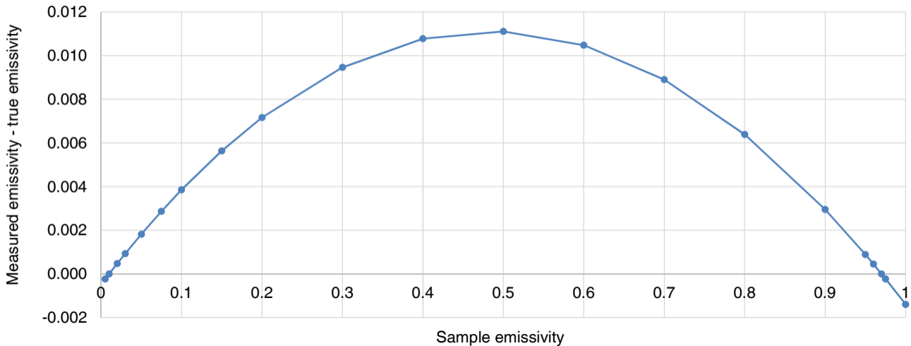
TIR100-2 - Error on measured near-normal emissivity due to multi-reflections for diffuse surfaces Hemisphere emissivity = 0.91
