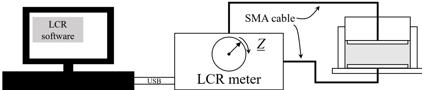
(a) System architecture of the measurement setup
