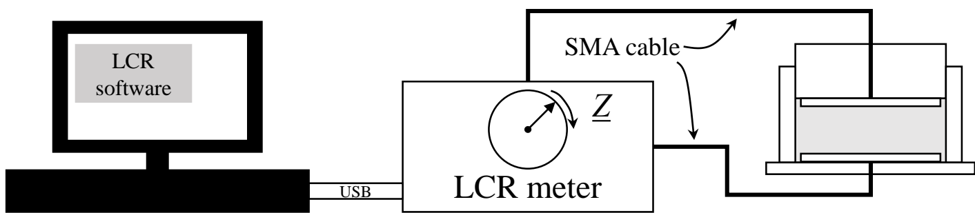
(a) System architecture of the measurement setup
