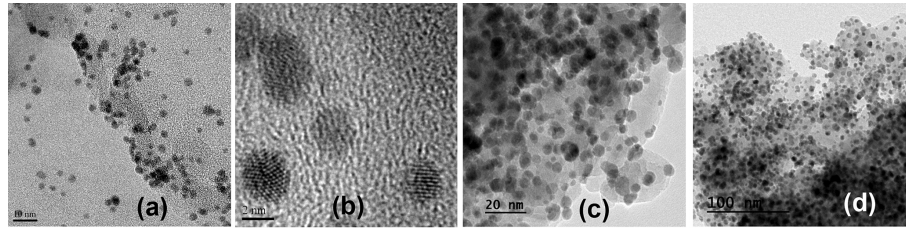
Figure 1. TEM micrographs of catalyst A: (a) and (b); catalyst C: (c) and (d).
