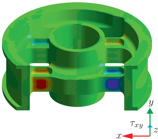
Loadcase with force F_z
