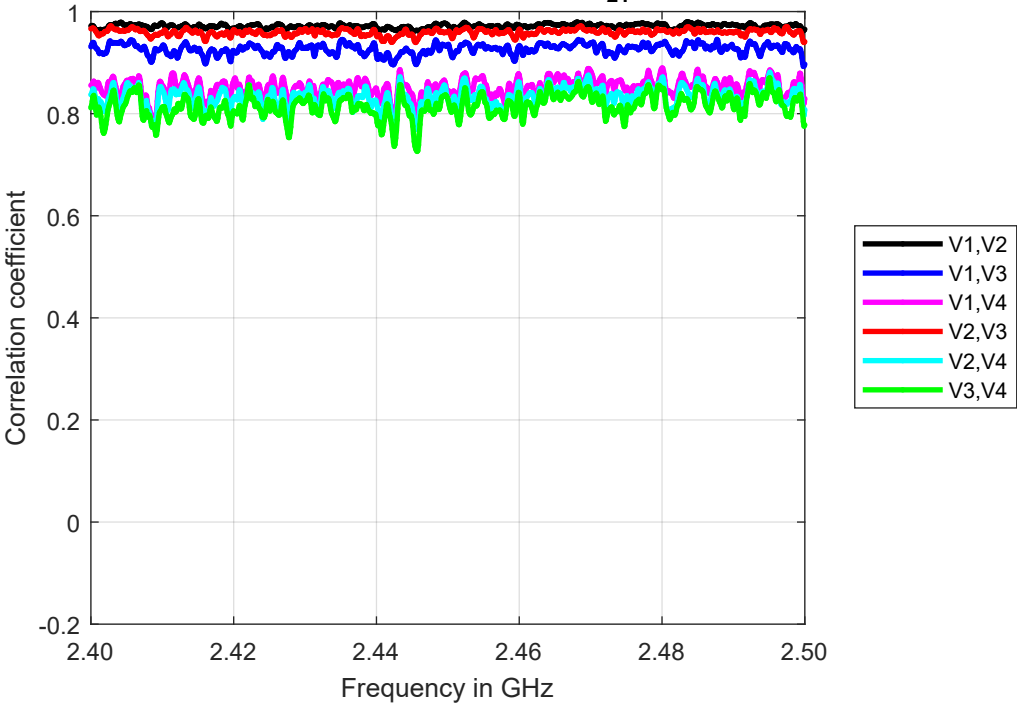
Correlation coefficients of |S_{21}|^2
