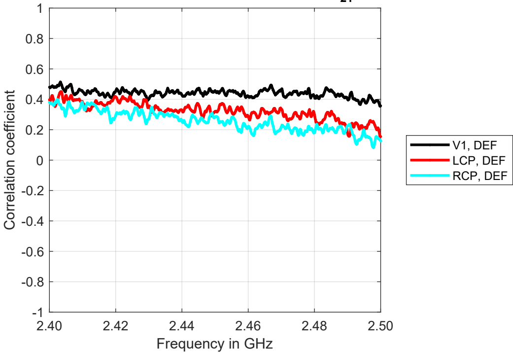
Real part (compl. correlation coeff. of S_{21} )
