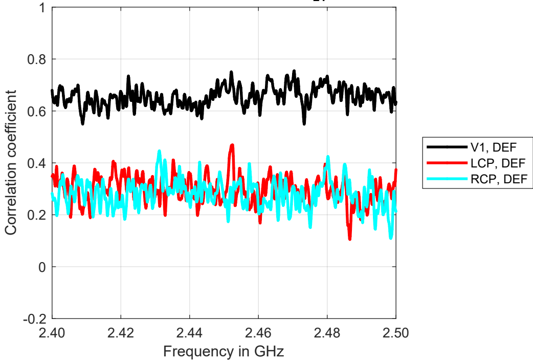
Correlation coefficients of |S_{21}|^2
