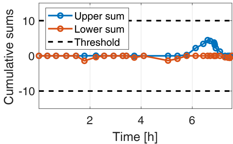
CUSUM control chart
